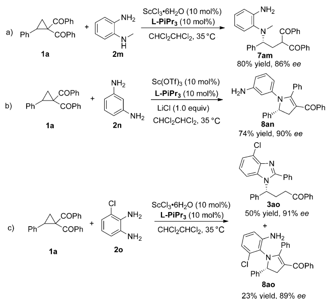
Scheme 3. Control experiments.
